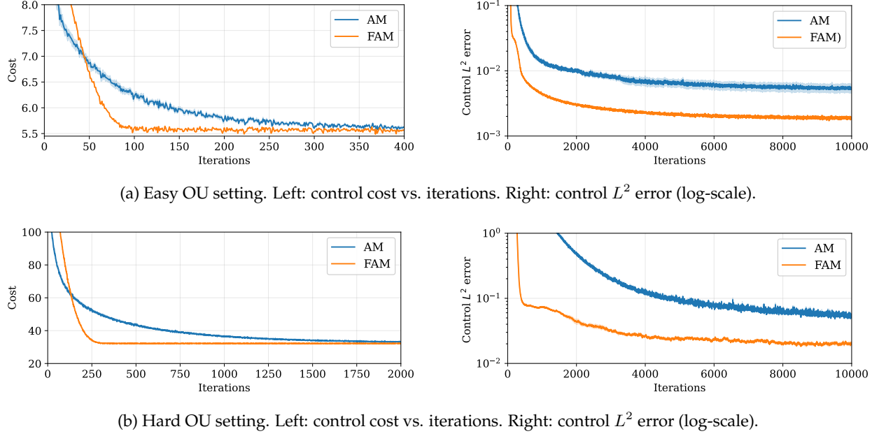
Figure 2: Comparison of Adjoint Matching (AM) and Fisher Adjoint Matching (FAM) on quadratic Ornstein-Uhlenbeck control problems. Solid curves show the mean over three seeds and shaded regions indicate one standard deviation. FAM achieves faster convergence and lower control error, particularly in the harder regime.
