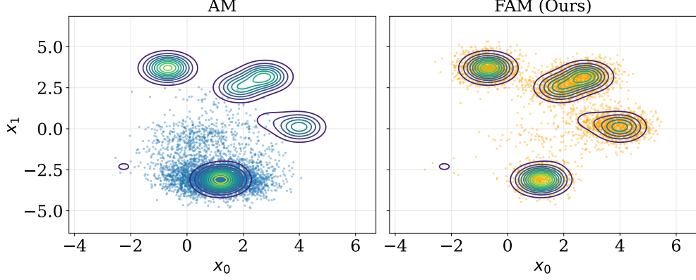
Figure 1: Qualitative comparison on a 2D GMM target. Contours show the ground truth density; dots are samples at iteration 500. AM exhibits slow convergence, while FAM successfully captures all modes after less iterations. Left: AM baseline. Right: FAM (ours).
